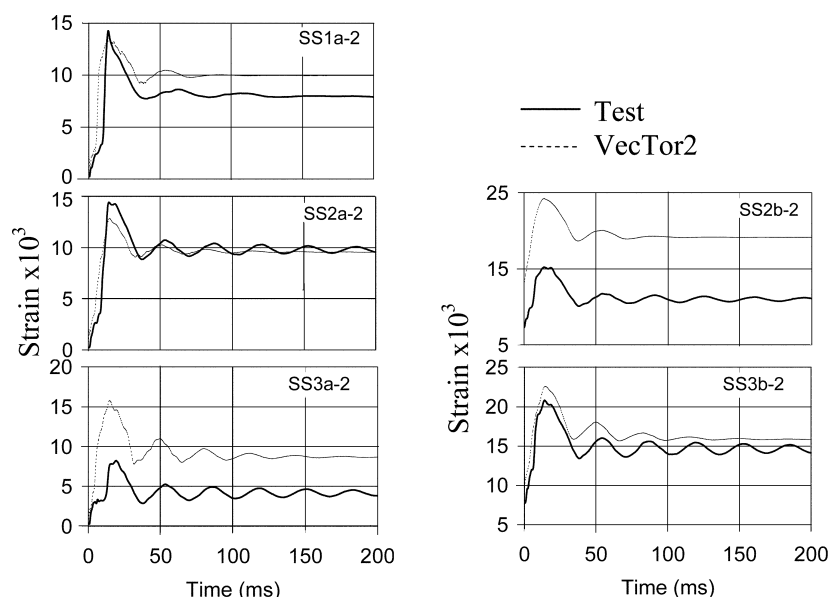
Fig. 11—Observed and calculated longitudinal reinforcing bar strains at midspan, second impacts.
