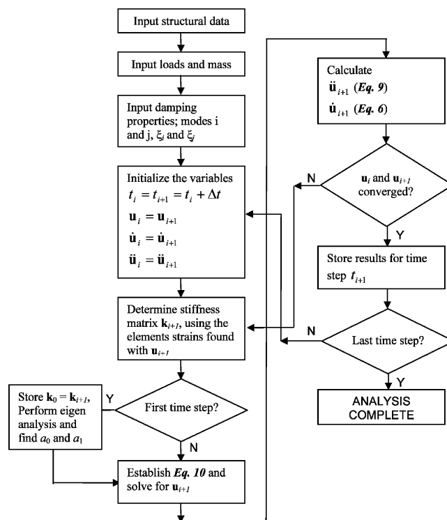
Fig. 1—Flowchart for proposed NLFEA procedure.
