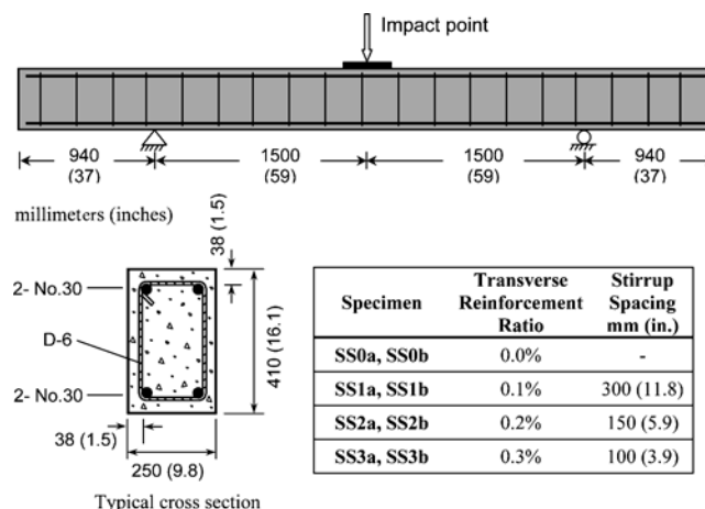
Fig. 2—Specimen properties.
